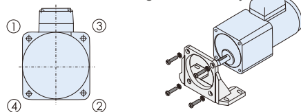
与直角安装脚组合 Combination with right-angle mounting feet
